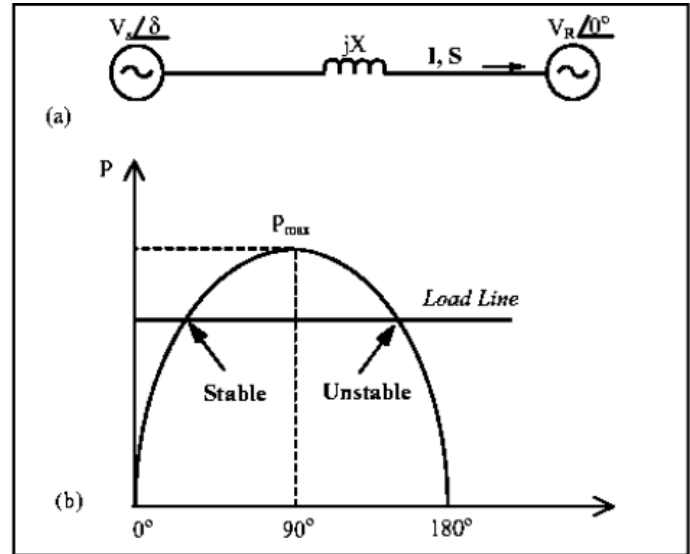
Figure 2.2.1: Model for Calculation of Real and Reactive Power flow
