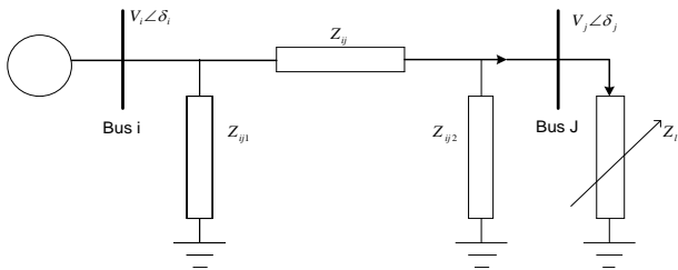
Figure 3.1.2.2 Equivalent circuit of Fig 3.1.2.1
