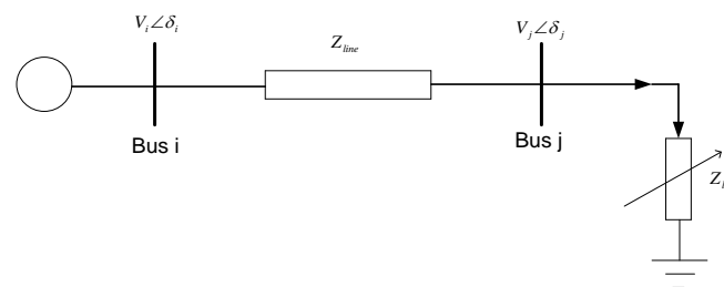
Figure 3.1.1 Simple two bus system to determine LVSI
